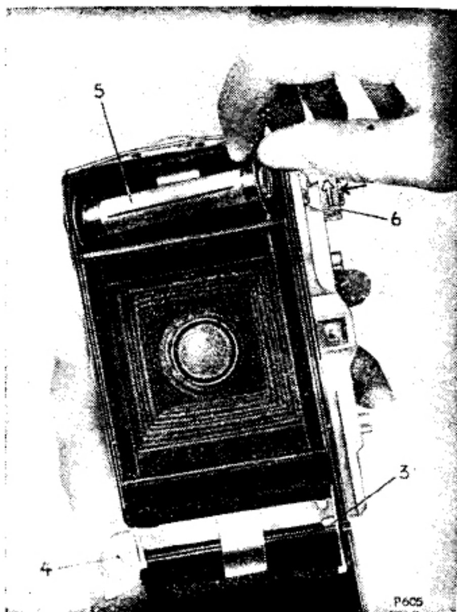
Fig. 16 Placing the empty spool
