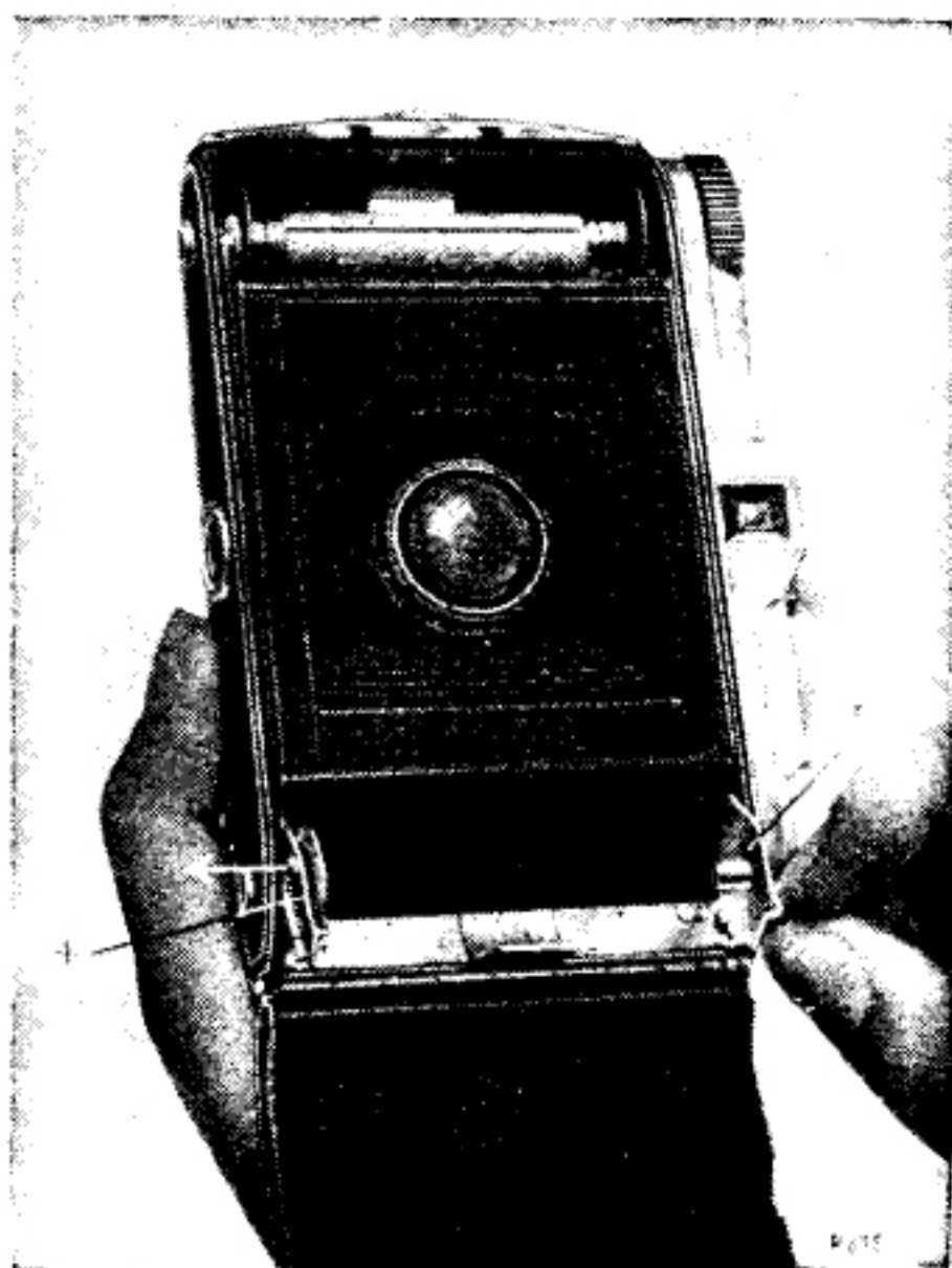
Fig. 2 Swinging out the spool-holder
