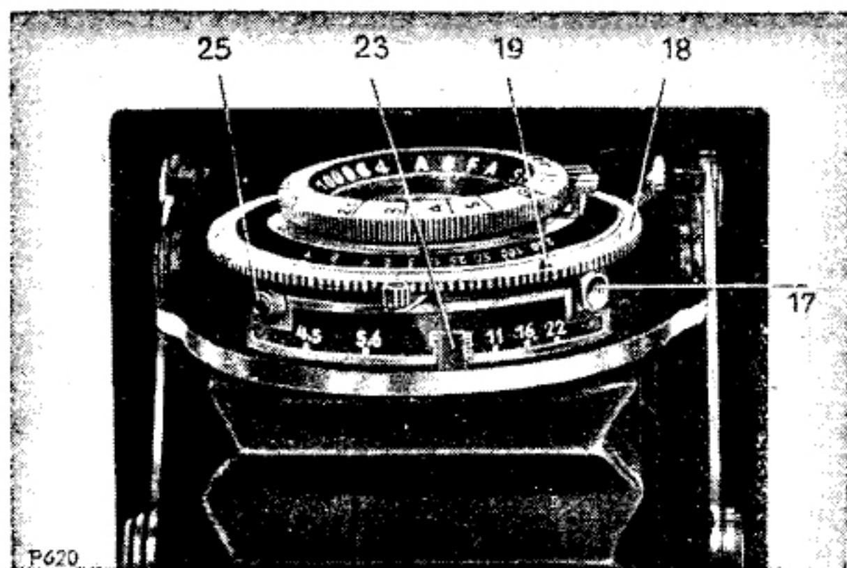
Fig. 12 Setting the lens aperture
